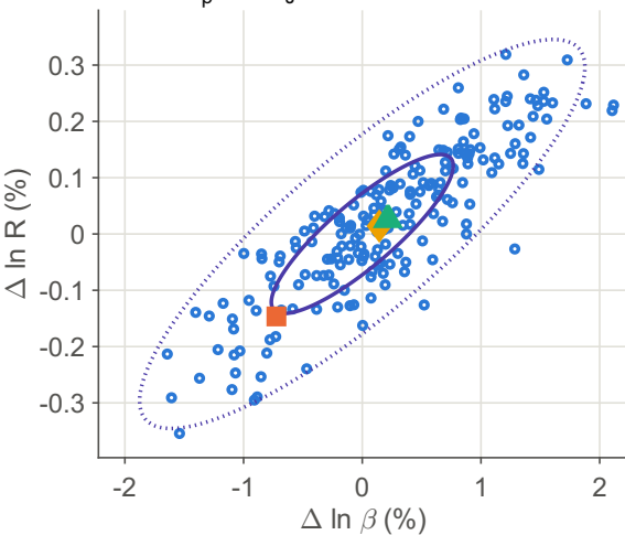
(c) R2: \omega_p 3.5, \gamma_J 7 ( n = 200 )
